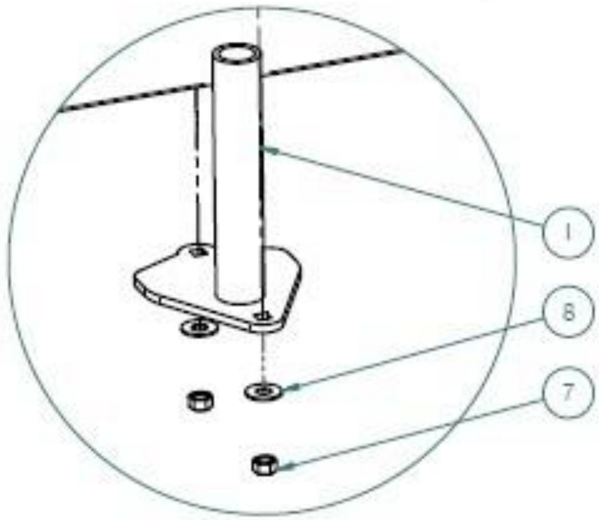
DETAIL A
